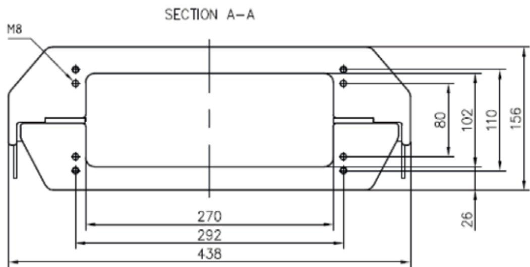
Blind flange up to 6.6 kV.
