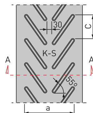
Blow-up view of a rib
